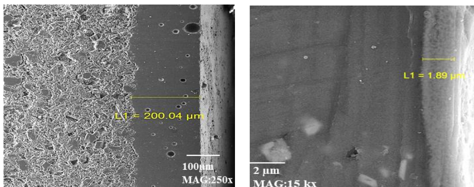
Fig. 7. Cross-section of Photocatalyst-coated glazed tile with ST-15B composition
